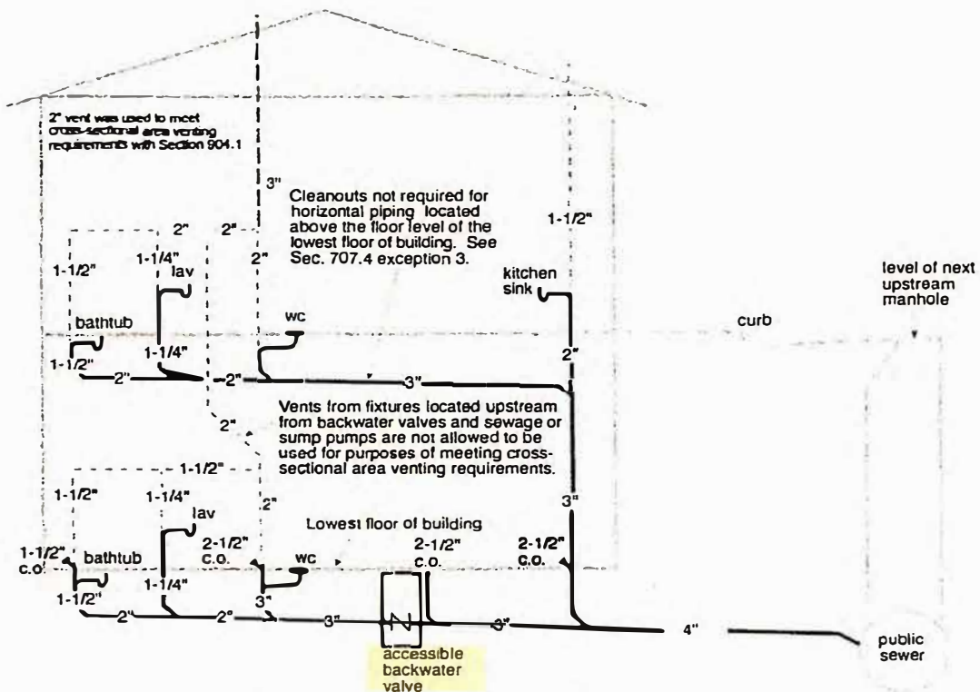
Figure 7-23 Fixtures Located Below Upstream Manhole Cover
